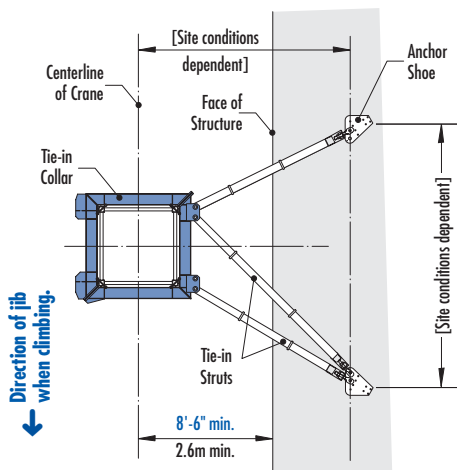
TIE-IN ASSEMBLY (Plan View)
